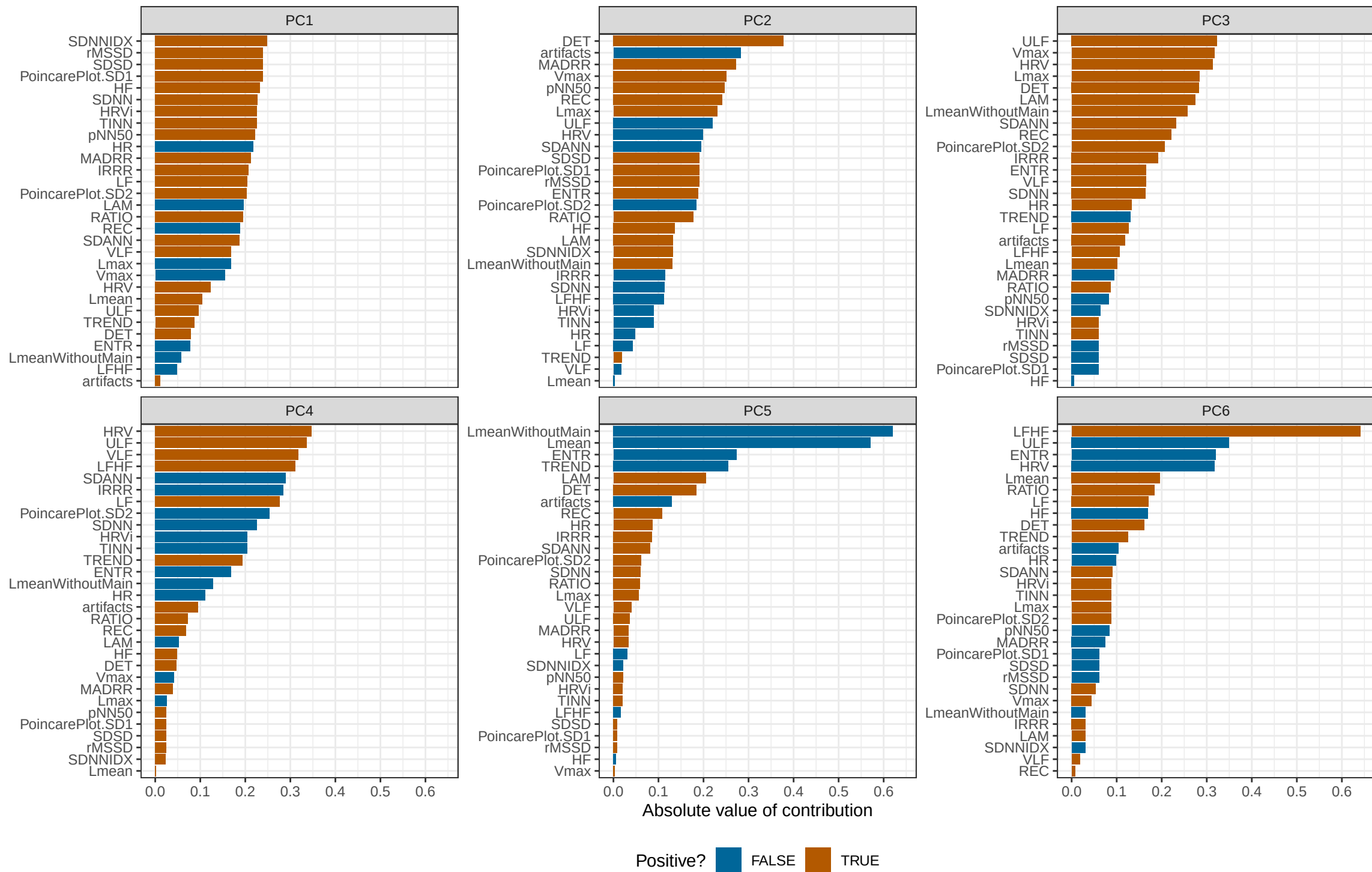
Loadings plot of the first 6 principal components of PCA for FLARE003
